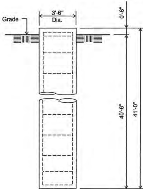
ELEVATION VIEW (14.6 cu. yds.) (3 REQUIRED; NOT TO SCALE)
