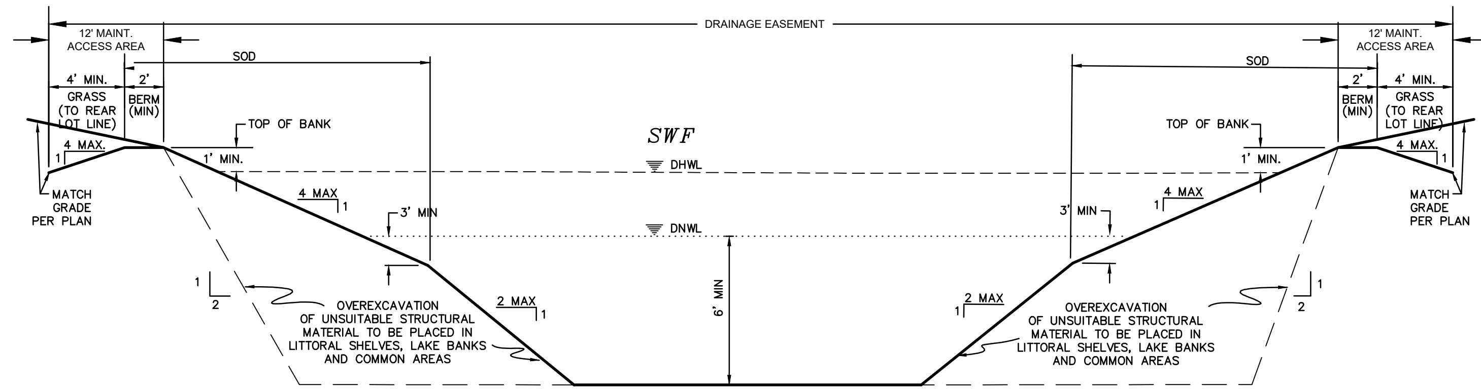
TYPICAL SWF SECTION
